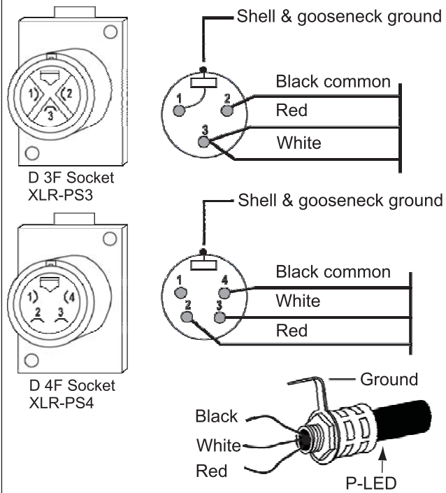
Figure C LED Wiring
